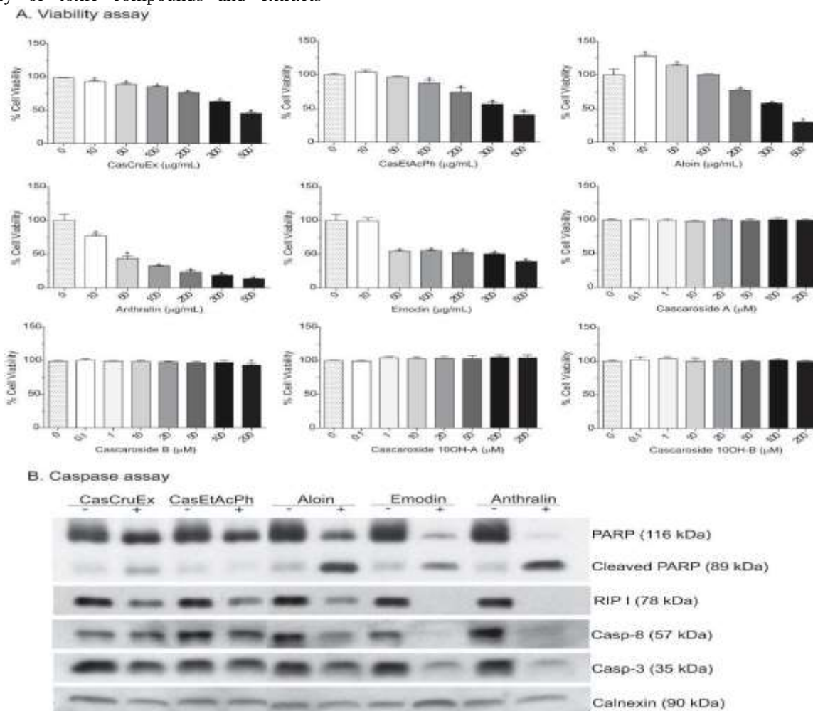
Figure 1: (A) Cell viability of NOK-SI cells at different concentrations of extracts and isolated compounds from cascara sagrada by alamarBlue viability assay. (B) NOK-SI cells were incubated with 300 \mu M of each compound (Aloin, Emodin and Anthralin) or extracts (CasCruEx and CasEtAcPh) for 48 h. Caspase-8, caspase-3, PARP and RIP1 proteins were
